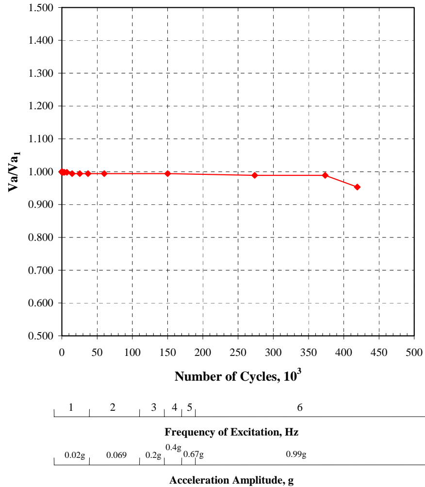
Ratio of Air Volume in the Specimen to the Initial Air Volume
