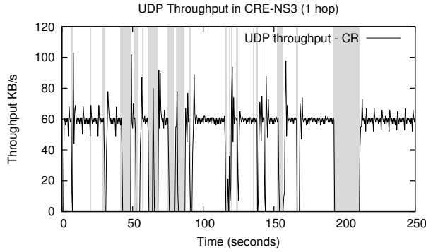
Fig. 5. UDP flow’s throughput vs. time in a CR network. Gray areas indicate PU activity.
