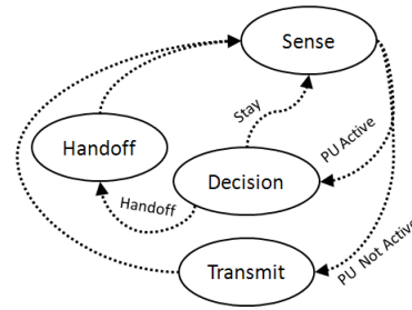
Fig. 4. State machine of the RX interface
